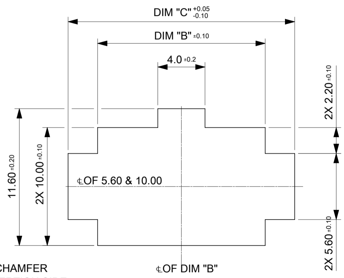
RECOMMENDED PANEL CUT-OUT DIMENSIONS PANEL THICKNESS 0.80-2.00MM
