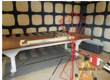
Radiated emission set-up (Vertical BICON test in a single DUT mode)
