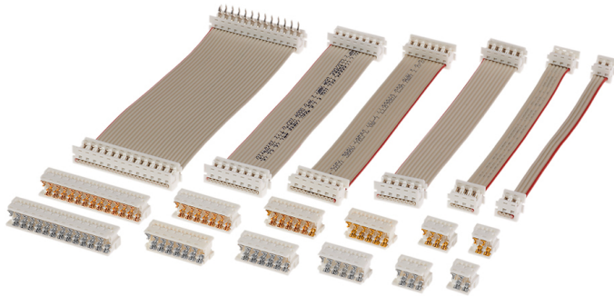
Picoflex Ribbon Cable Assembly
